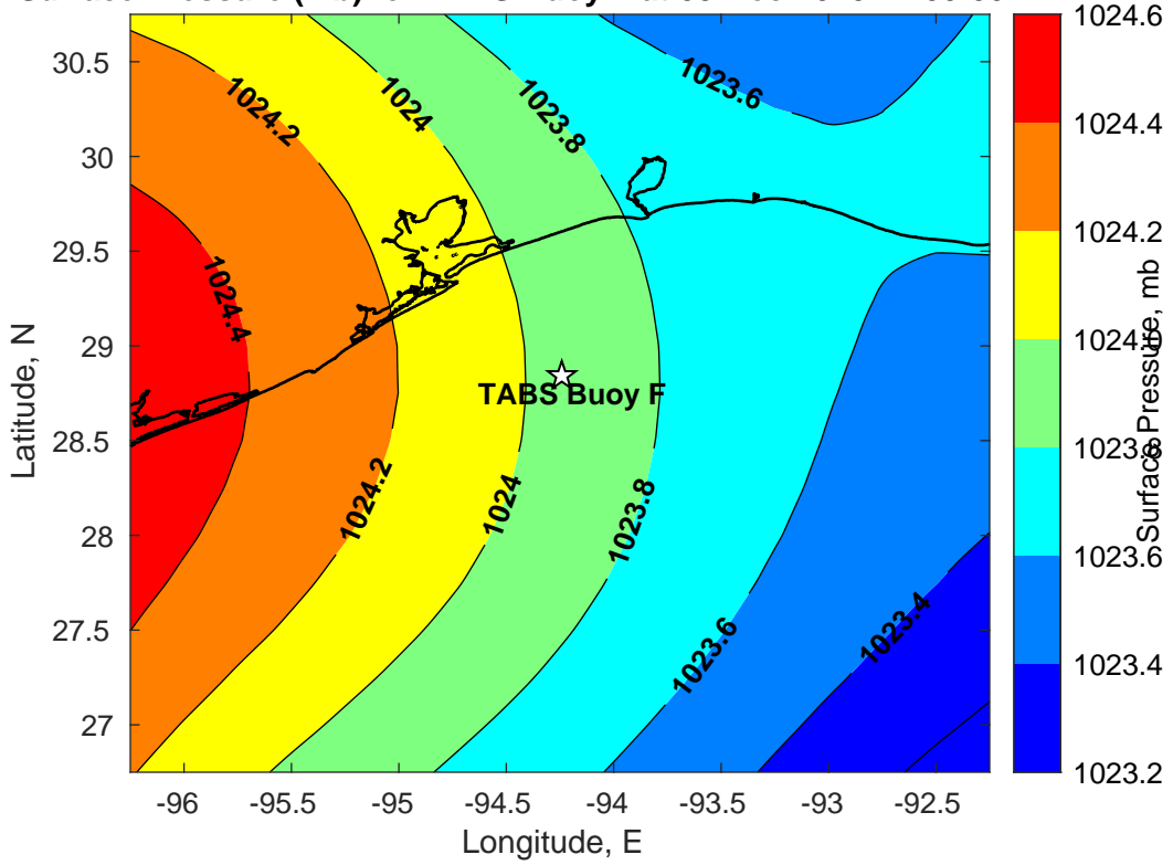
Surface Pressure (mb) for TABS Buoy F at 08-Dec-2020 12:00:00
